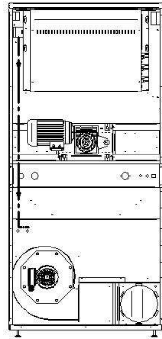
Rear view of the dryer.
