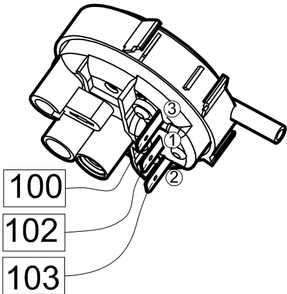
Pressure switch
