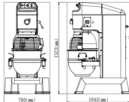
(SP-62P/SP-B62P) DIMENSION
